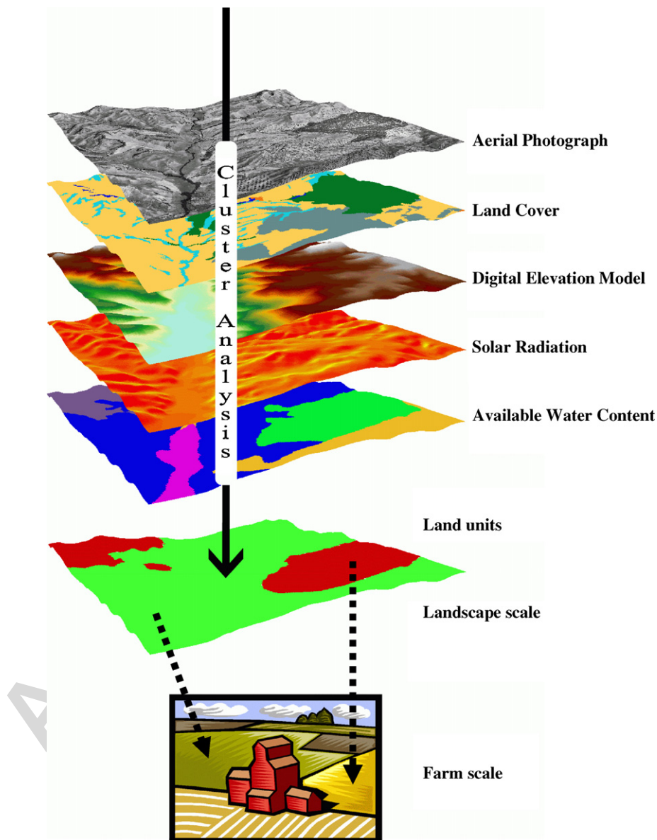
Fig. 2. GIS landscape data processing for each landscape test site (LTS) to create homogeneous land units (LU), corresponding to different qualities of agricultural land of a farm (Torrijos LTS example).
