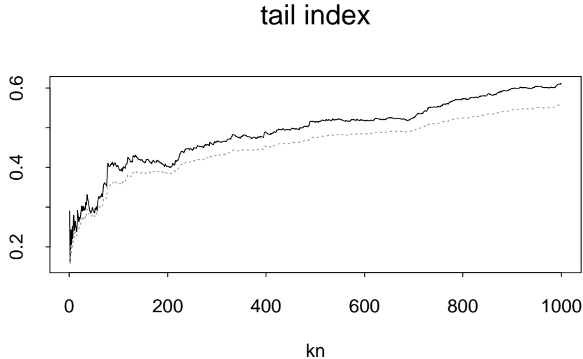
Figure 2: Tail estimates for Nedlloyd data. The dotted line stands for the alternative estimator used in the bootstrap.
