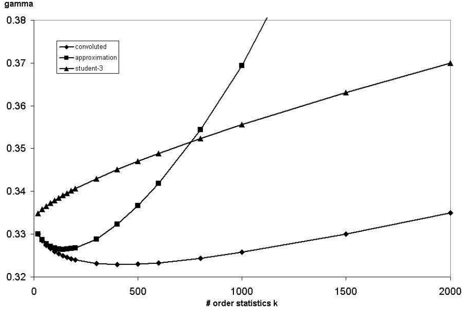
Figure 1: Theoretical Hill plot; sample size 100 000.
