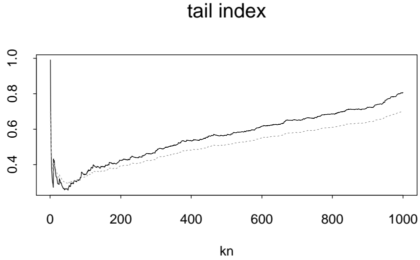
Figure 3: Tail estimates for Alcatel data. The dotted line stands for the alternative estimator used in the bootstrap.
